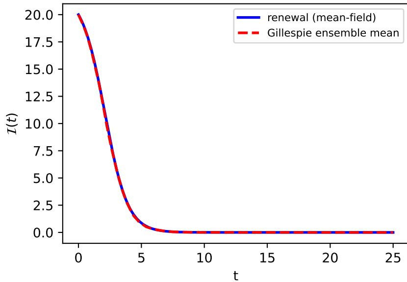
Infected cells (mu0)
