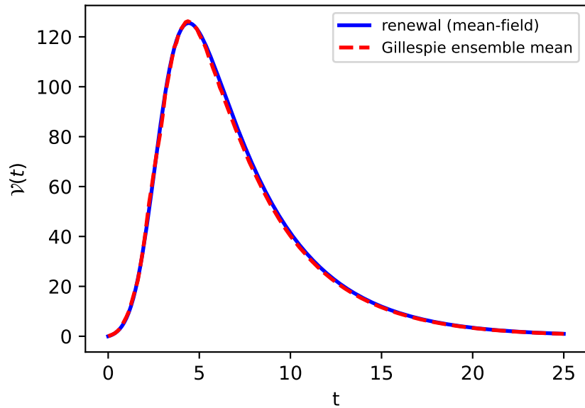
Free virus (mu0)
